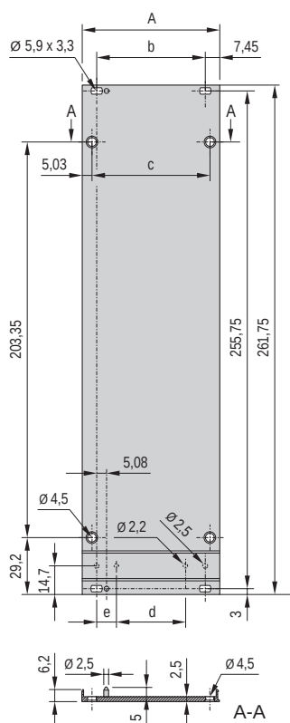
6 U Front panel shielded
