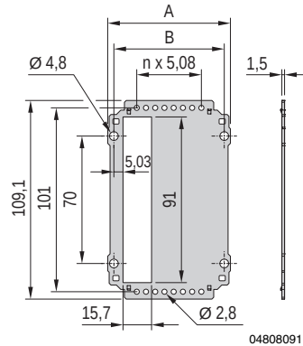
For single connector
