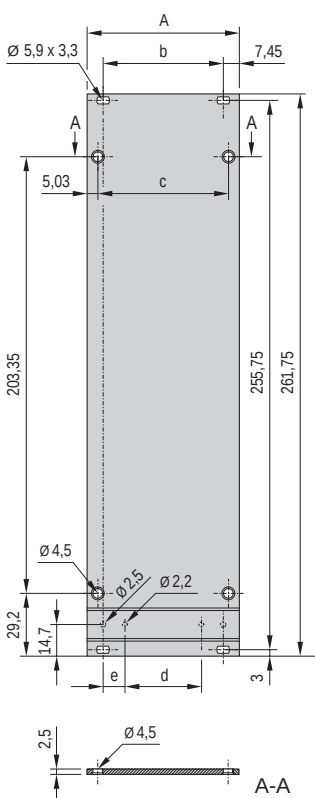
Front panel unshielded
