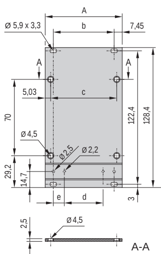
Front panel unshielded
