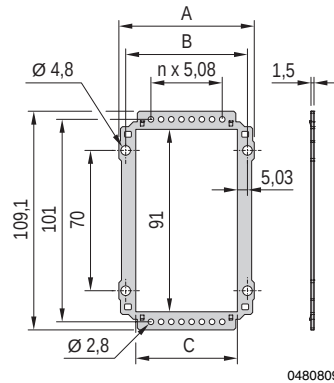
For multiple connectors
