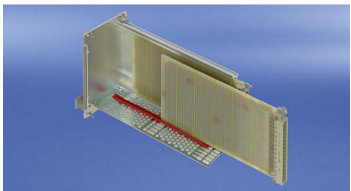
Board fixing in slot 1 on side panel, in all other slots board fixing with guide rails
