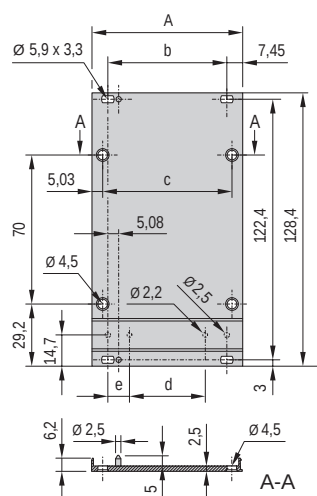
3 U Front panel shielded
