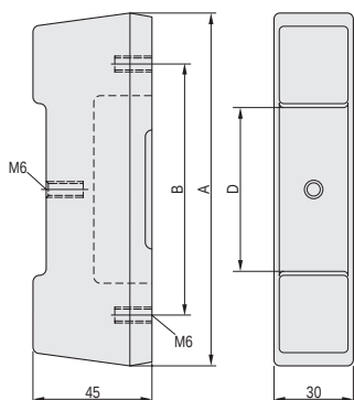
Dimensions for modify the rear panel
