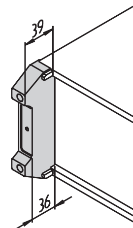
Foot for rear hood
