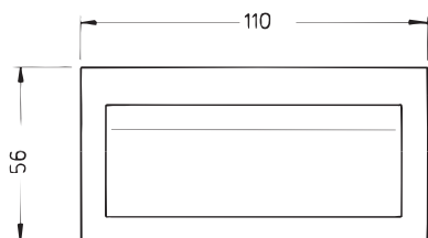
Size 1, case cut-out 49 × 104 mm
