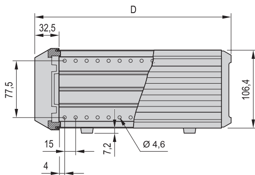
Cross-section 2 U, 3 U
