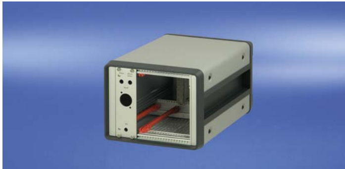
Application: ratiopacPRO-air case in special colour, shielded board cage, air filtered fan top and bottom
