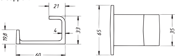
Cable support
