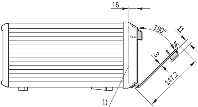
1) Front panel
